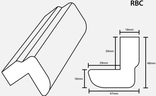
Round Bullnose Cornice
