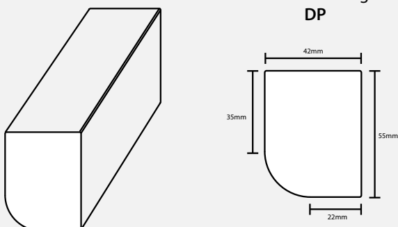
Dual Purpose Cornice
