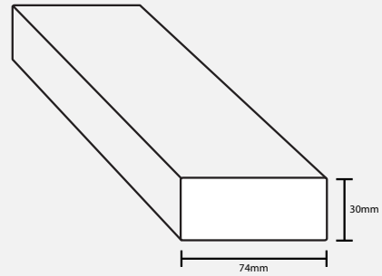
Square Edged Moulding
