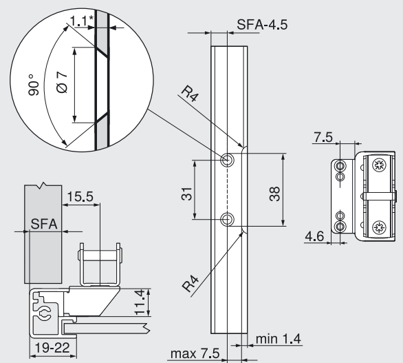
Narrow aluminium frames Wooden fronts and wide aluminium frames 1)
