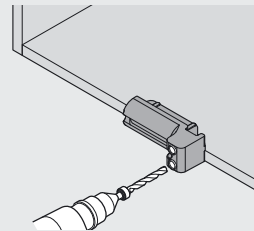
TIP-ON drilling template
