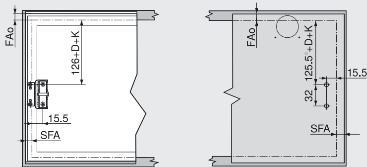
Narrow aluminium frames Wooden fronts and wide aluminium frames 1)
