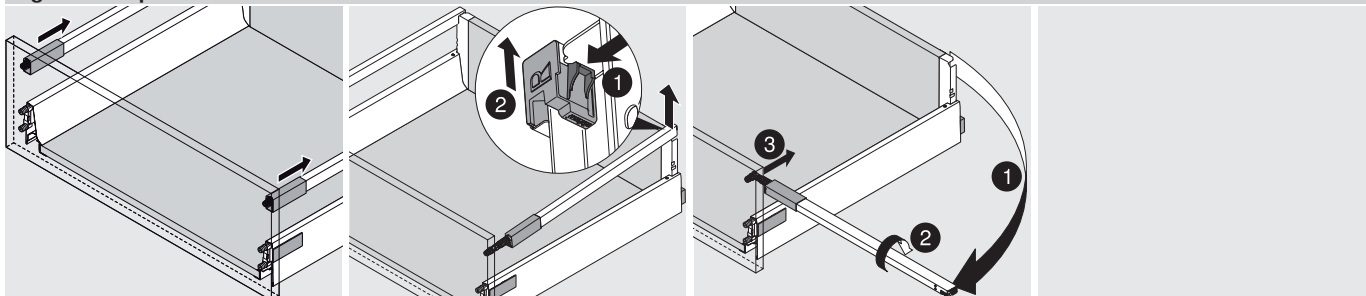
Removal
