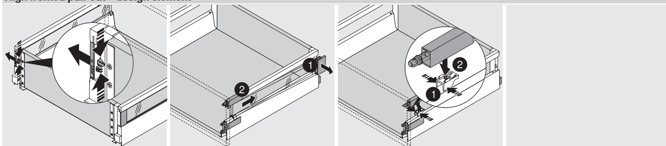
Removal
