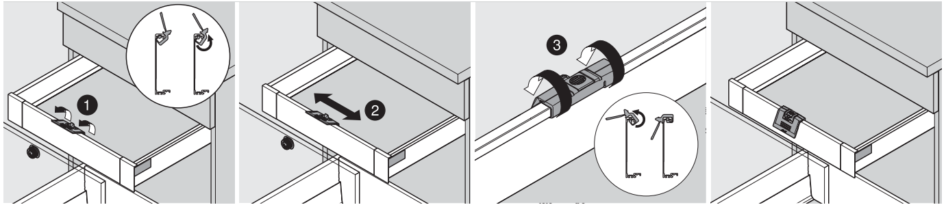
Assembly
