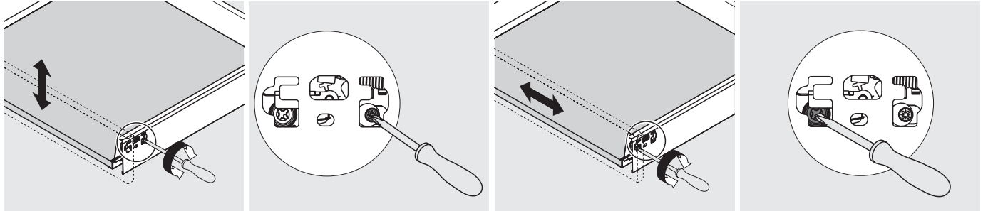
Height adjustment
