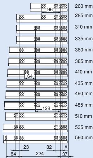
Hole pattern 561H
