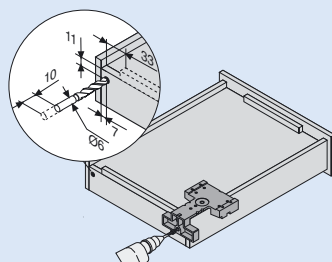
Drawer drilling jig (hook)
