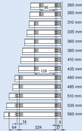
Hole pattern 551H
